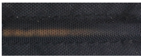
1h at 220°C on the heating cable: the PA66 starts to change color
