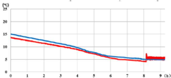
Variation of the water temperature in the container, while the ambient temperature is -10^{\circ}C , with a surface load of 0.05 W/cm^2 (150W). It can be seen that the internal temperature of the container stabilizes at 5^{\circ}C .
