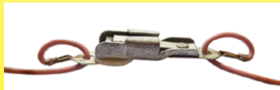
Calor slow-break heating blanket temperature limiter, calibrated at 80°C (circa 1960). Note the waterproof PVC sleeve welded on the wires and the loop made by the electrical conductors passing through a hole in each terminal- this is to eliminate tensile stresses on the wire (Ultimheat Collection)
