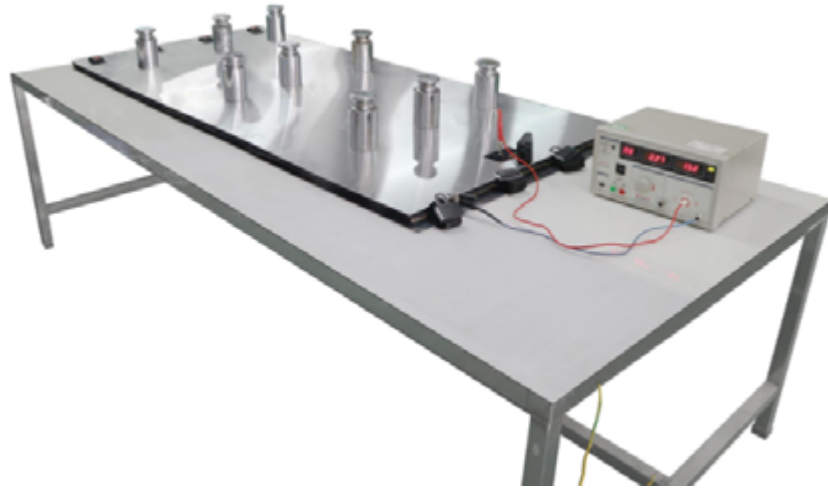
Measuring equipment for total current leakage at cold condition
